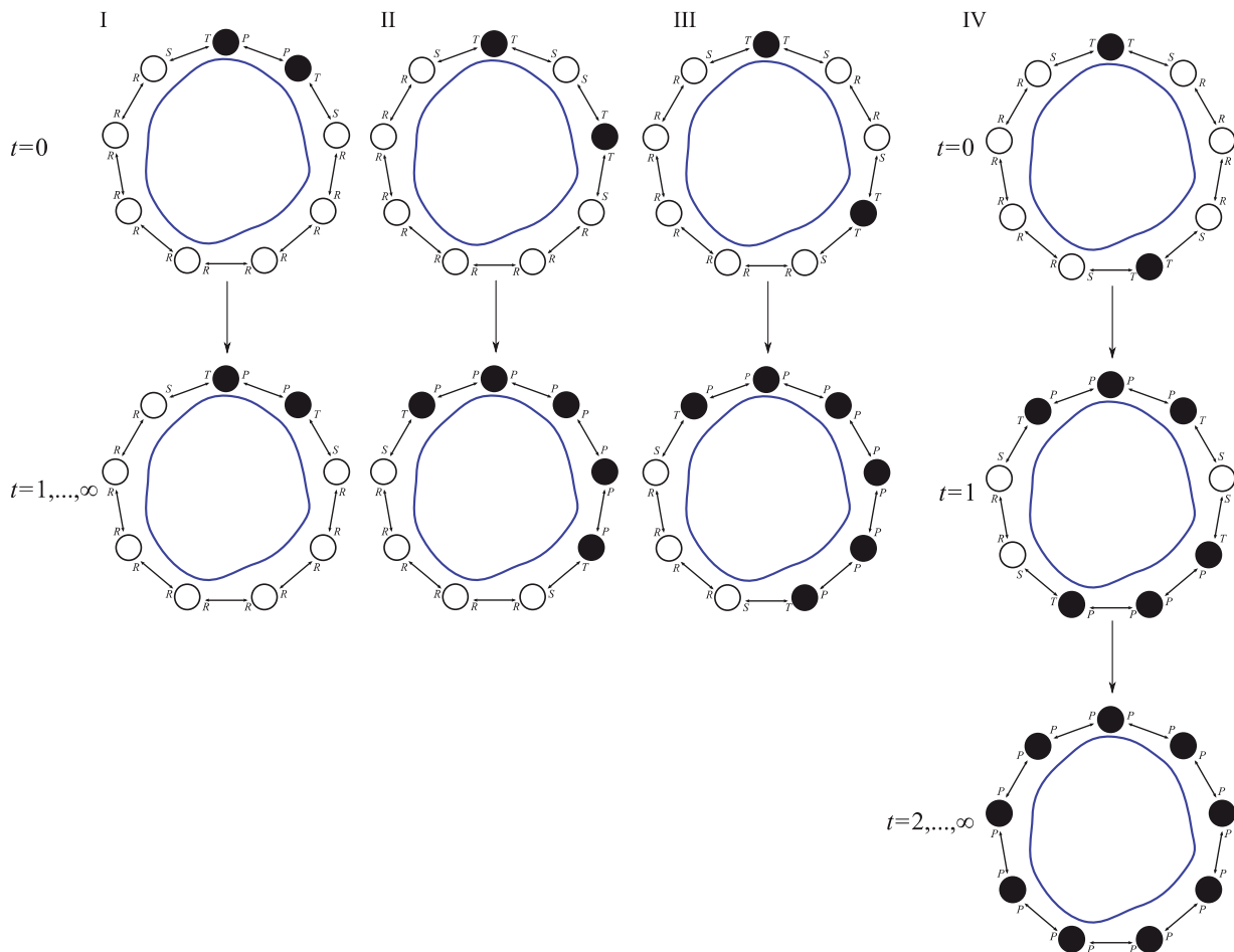
Fig. 3. The evolution of strategies in a settlement of n = 9 farmers in the wake of two random mutations.
