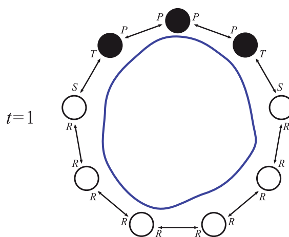
Fig. 2. Strategies and payoffs in a settlement of n = 9 farmers, in generation t = 1 , and in the wake of one mutation.
