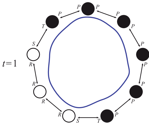
Fig. 4. A configuration D_1(9, 6) = (0, 0, 0, 3, 0, 0) allowing the survival of cooperation in the settlers' village after an appearance of mutant defectors in the ancestral village according to configuration D_0^y .
