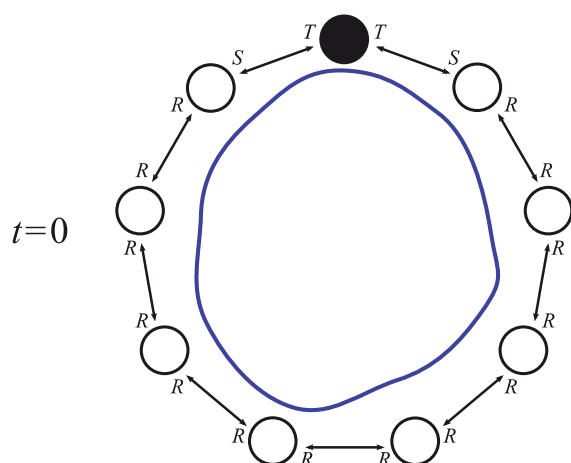
Fig. 1. The strategies and the payoffs in a settlement of n = 9 farmers, in generation t = 0 , and in the wake of one mutation.
